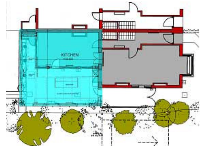
Ground Floor Plan Showing Extension in Blue
